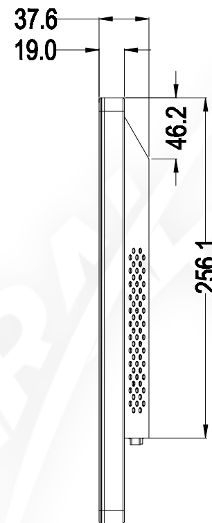
Side View
