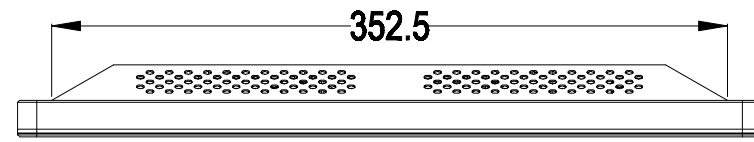
Top View
