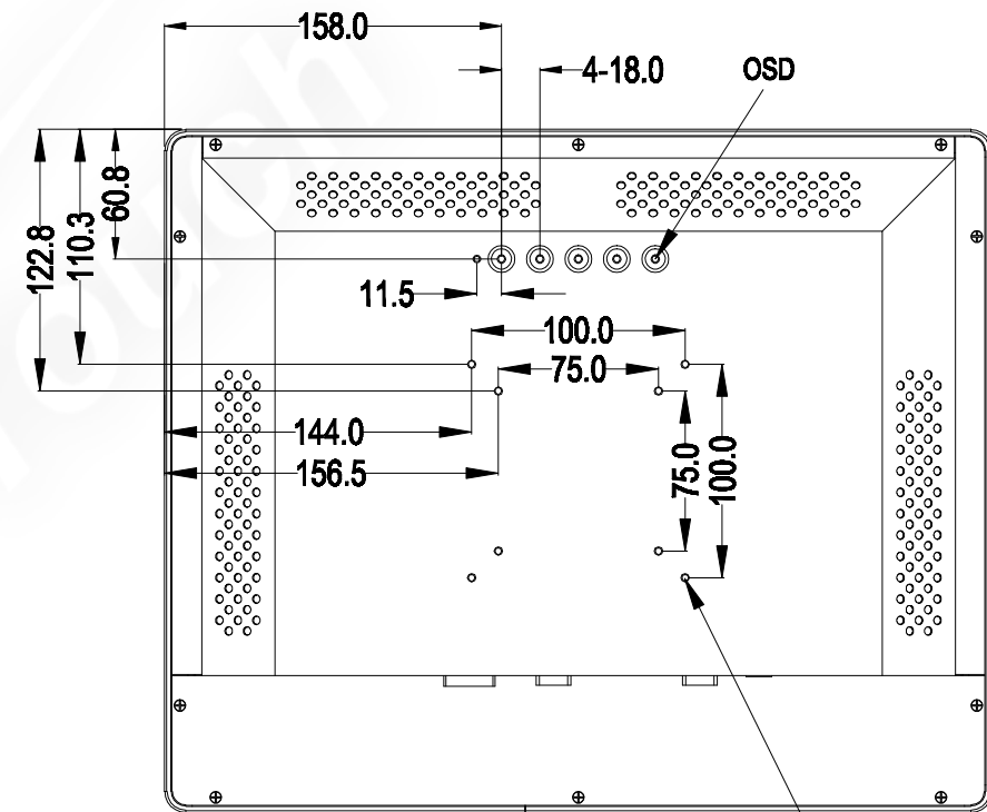
VESA MOUNT
